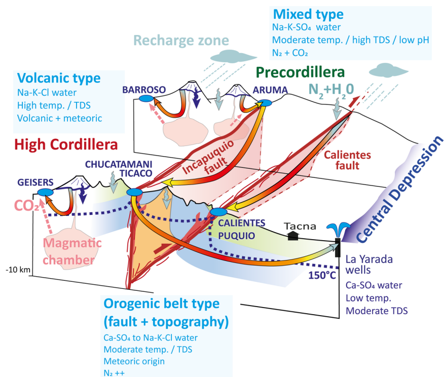
Figure 1: Conceptual model of the Tacna hydrothermal systems.
