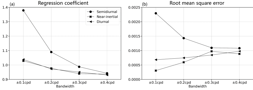
Figure 2. The (a) regression coefficient and (b) root mean square error ( \text{m}^2 \text{s}^{-2} ) between Lagrangian and Eulerian semidiurnal, near-inertial and diurnal KE as a function of bandwidths of \pm 0.1 cpd, \pm 0.2 cpd, \pm 0.3 cpd, \pm 0.4 cpd.
