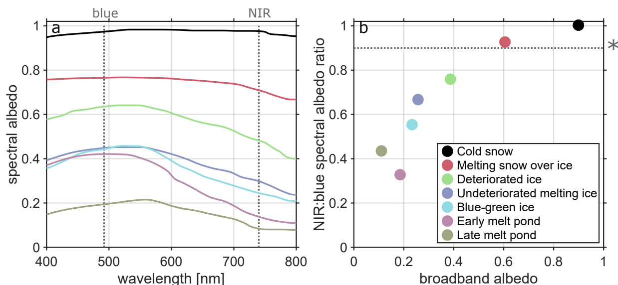
Figure 6. Spectral albedo a and the ratio between the spectral albedo in the near-infrared (NIR) and blue, or NIR:B b for a variety of classifications of first-year sea ice, organized by broadband albedo. Data shown in a were taken from Perovich (2017) and used to compute quantity shown in b . Asterisk in panel b indicates a NIR:blue ratio of 0.9.
