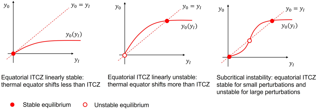
Figure 15. Schematic depicting the sensitivity of the thermal equator y_0 to the latitude y_I of ITCZ heating under idealized scenarios supporting linear stability (left), linear instability (middle) and subcritical instability (right). The filled (empty) red circles represent stable (unstable) equilibria.
