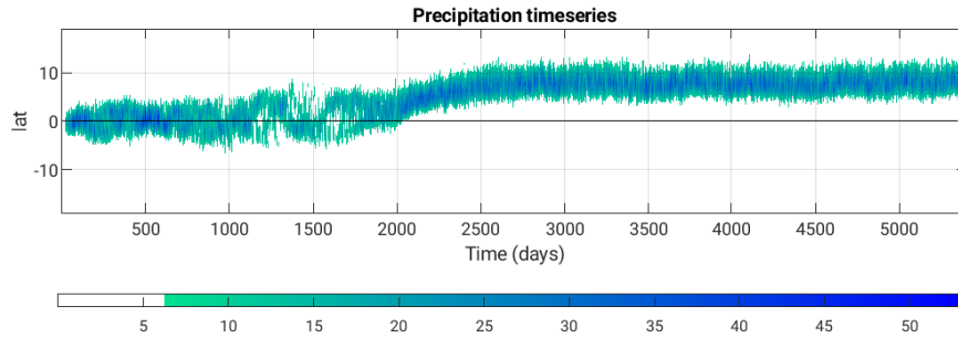
Figure 1. Time series of zonal-mean precipitation (mm/day) for a T85 simulation with no convective parameterization and a 20 meter deep slab ocean.
