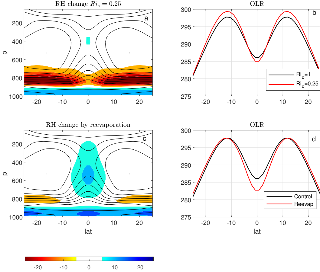
Figure 13. (a) Climatological relative humidity for the control swamp simulation with Ri_c = 1 (black contours every 10%) and RH changes when Ri_c is reduced to 0.25 for T85 resolution simulations; (b) OLR for the control swamp simulation (black) and for the simulation with Ri_c = 0.25 (red); (c, d) As above but when enabling rain reevaporation.
