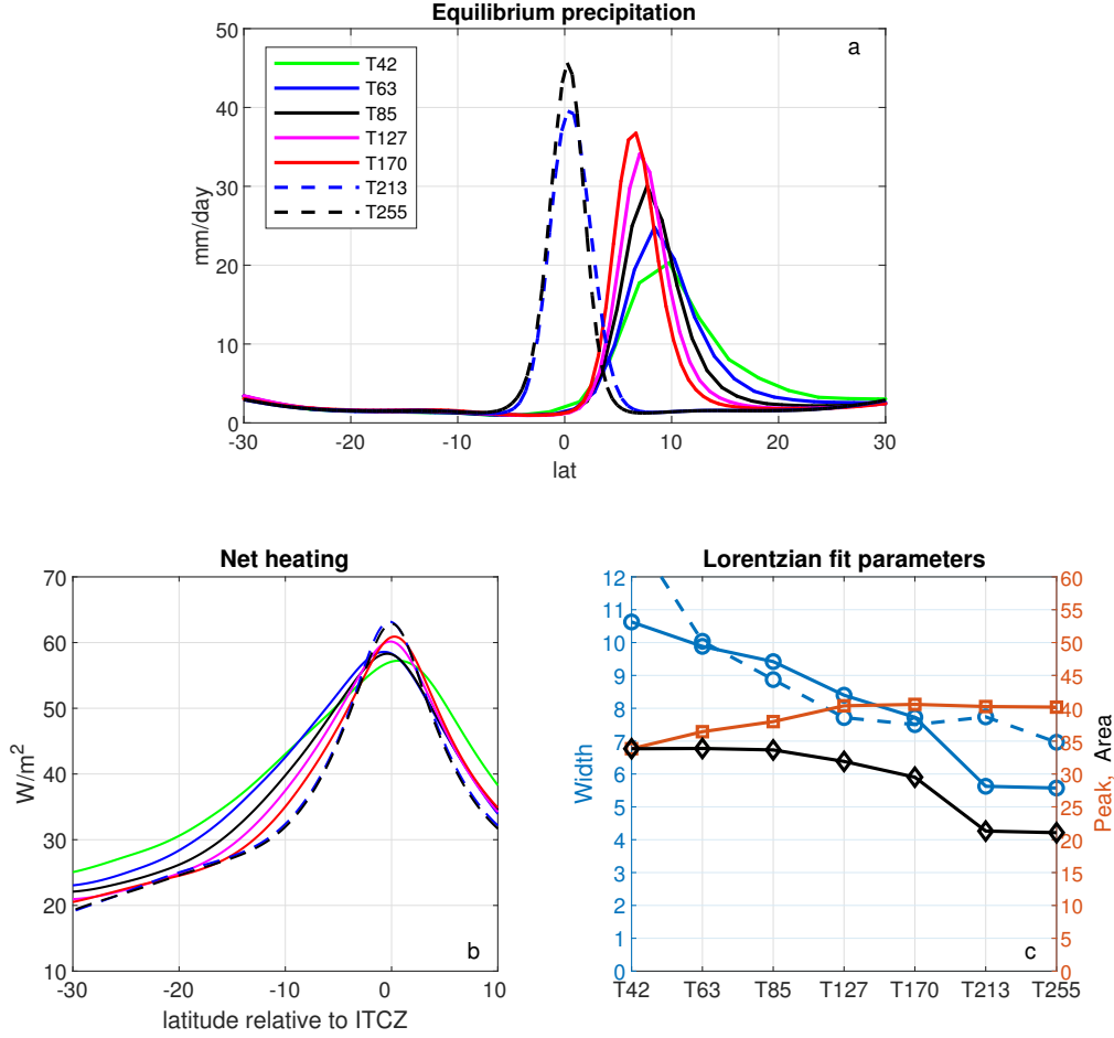
Figure 7. (a) Equilibrium zonal-mean precipitation for simulations with no convective parameterization at various resolutions (see legend). Solid/dashed lines are used to differentiate shifted/symmetric ITCZs. (b) Net heating for the same simulations as a function of distance to the ITCZ. (c) Resolution sensitivity of the Lorentzian best fits to the heating width w (blue) and amplitude s_I (orange) in Eq. 1, together with the normalized area ( s_I * w/w_{T42} , black). We also show with dashed line the width of the heating in the swamp setting.
