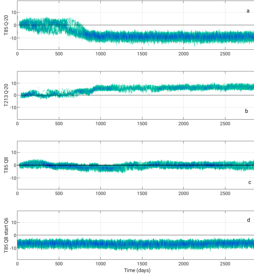
Figure 11. Timeseries of zonal-mean precipitation for: (a) A T85 simulation with poleward Qflux 20 \text{ W m}^{-2} ; (b) A T213 simulation with poleward Qflux 20 \text{ W m}^{-2} ; (c) A T85 simulation with equatorward Qflux 8 \text{ W m}^{-2} ; (d) Same as c but starting from the equilibrated climate obtained with an equatorward Qflux 6 \text{ W m}^{-2}
