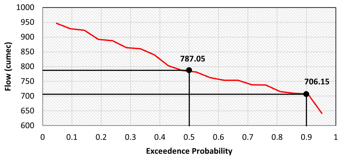
Flow Duration Curve of September Shitalakhya River SW 179
