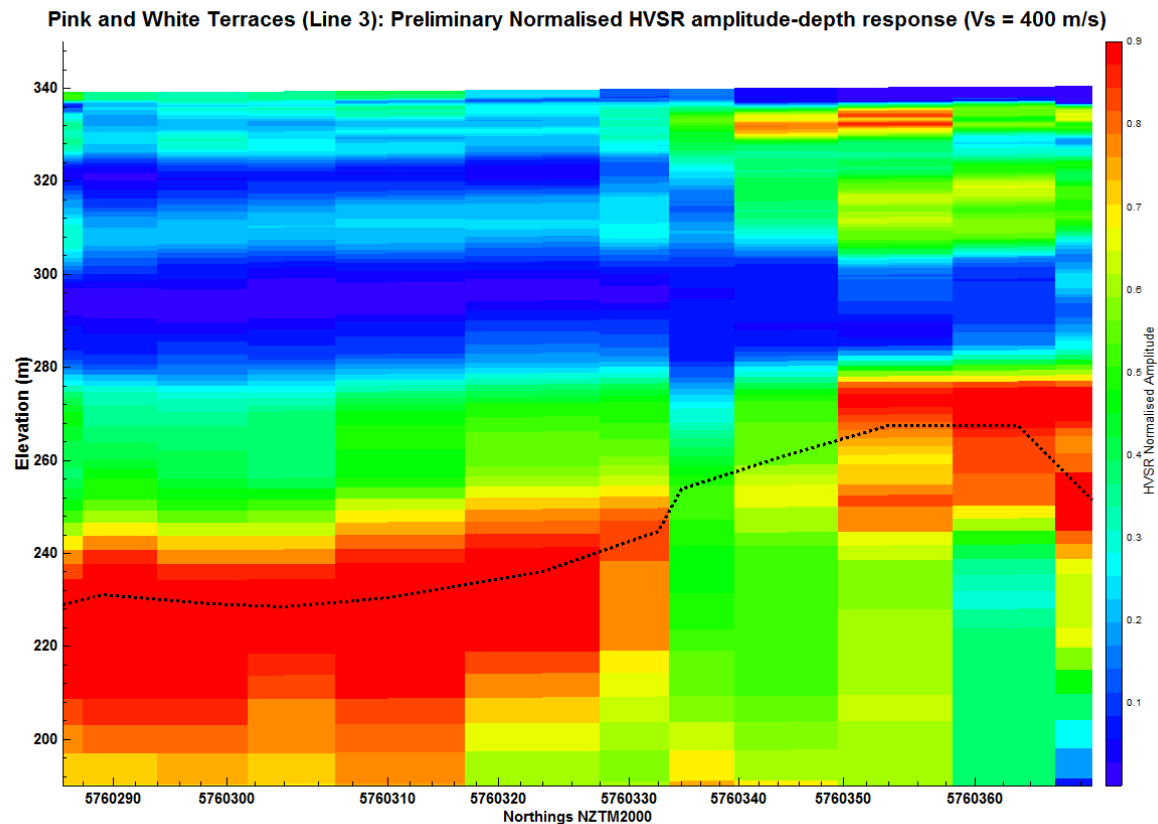
Figure 6. Overflow HVSR response ( V_s = 400 m/s), (Resource Potentials).
