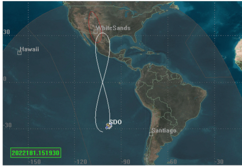
(a) The elongated figure-eight orbit as it is viewed by SDO's ground station.
