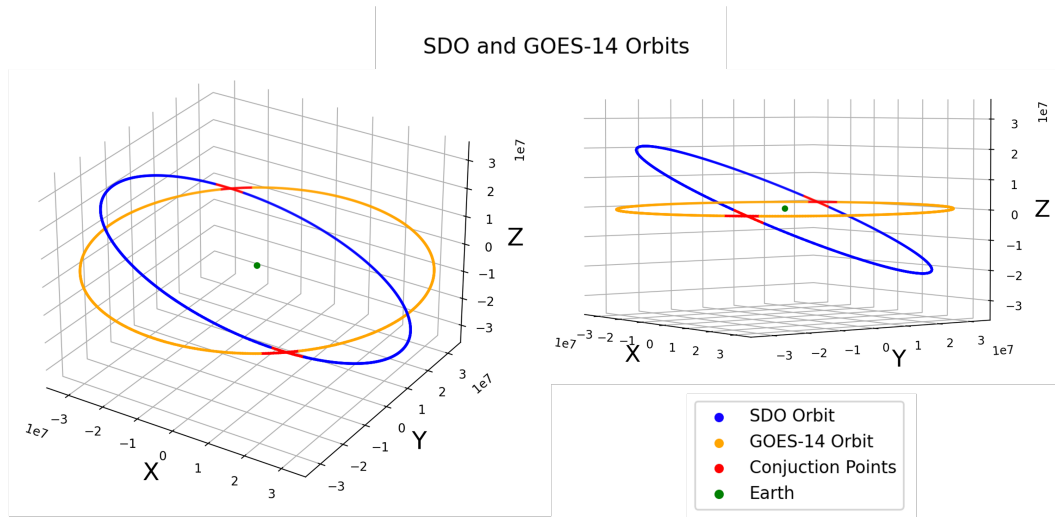
Figure 7: Three-dimensional plot of the SDO (blue) and GOES-14 (orange) orbits in the GEI coordinate system. In red are the conjunction parts of the orbits ( z_{SDO} = \pm 2,000 km) and in green is the center of the coordinate system, the Earth.
