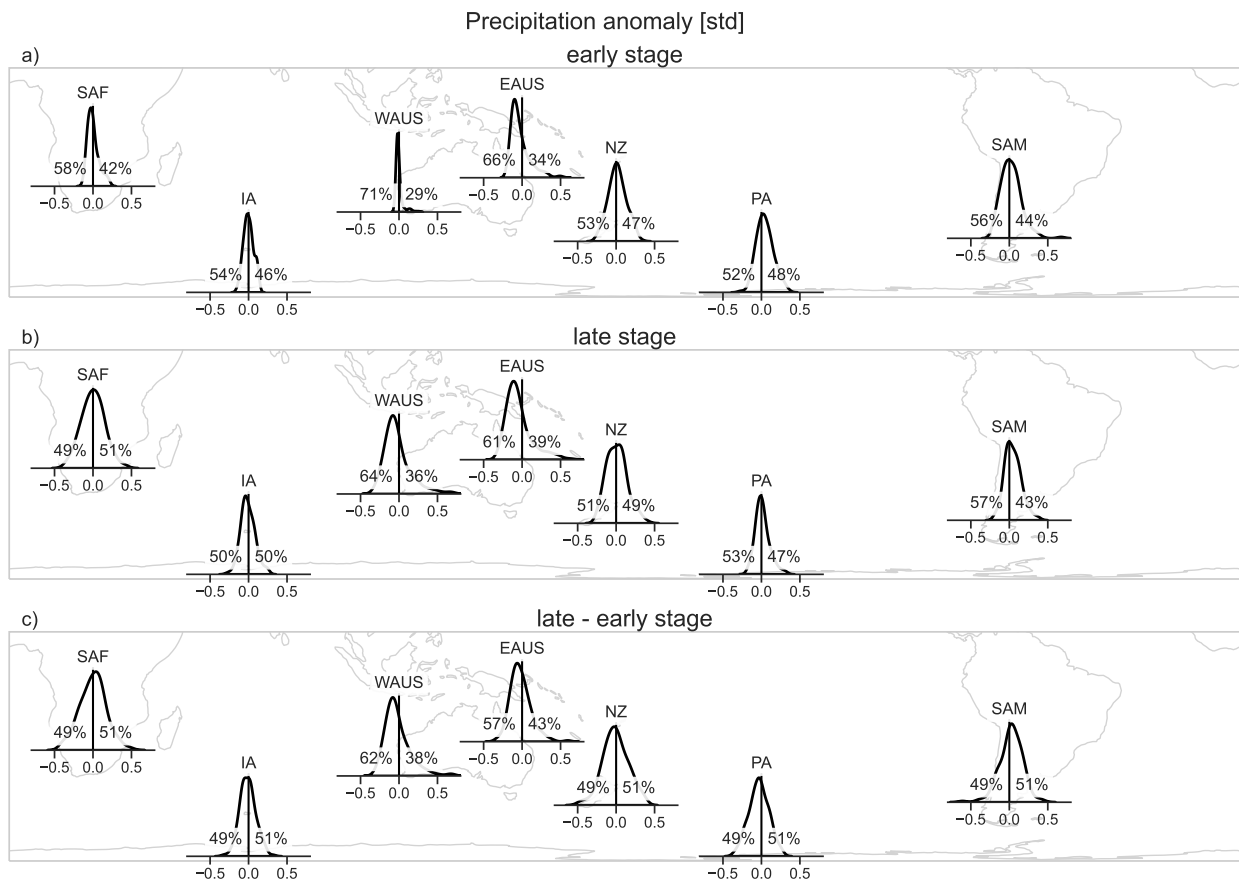
FIG. A2. Same as Fig. A2 but for years without SSWs. Given the PDFs show anomalies, their mean values are all zero and are therefore removed from the inset titles.
