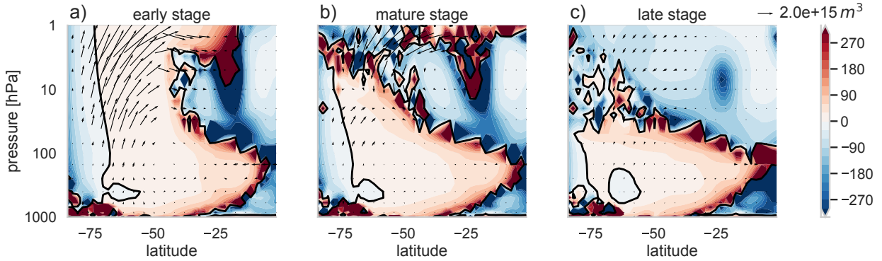
FIG. 9. Refractive index n^2 (shading) and flux vector anomalies (arrows) for (a) early, (b) mature, and (c) late stages and for wavenumber 1 waves. The black line denotes n^2 = 0 , arrows are computed and scaled following Jucker (2021b) and scale is indicated by the arrow on the right.
