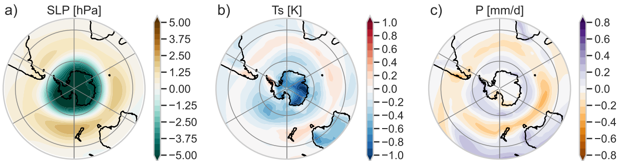
FIG. B1. (a) First Empirical Orthogonal Function of sea level pressure, whose Principal Component (PC1) serves as Southern Annular Mode index for this figure. (b) Regression of PC1 onto surface temperature, and (c) precipitation. These panels are produced with monthly model data and can be compared to Southern Annular Mode impact studies, such as Gillett et al. (2006), revealing a faithful reproduction of the SAM and its teleconnections in our model.
