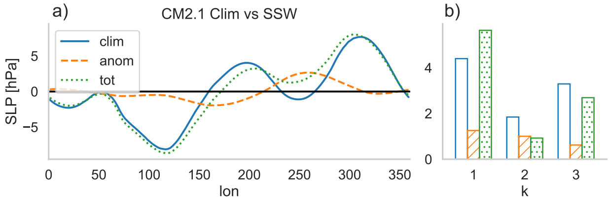
Fig. 2. (a) Zonally asymmetric sea level pressure (SLP) averaged between 70°S and 50°S for (blue) August-September climatology, (orange, dashed) early stage SSW anomaly, and (green, dotted) climatology plus anomaly. (b) Leading Fourier amplitudes (wavenumbers 1-3) for the same quantities. The strong SLP anomaly visible in Fig. 1a related to the Amundsen Sea Low (ASL) is located around 250°E, and corresponds to a weakening of the climatological low, which strengthens the global wavenumber 1 forcing.
