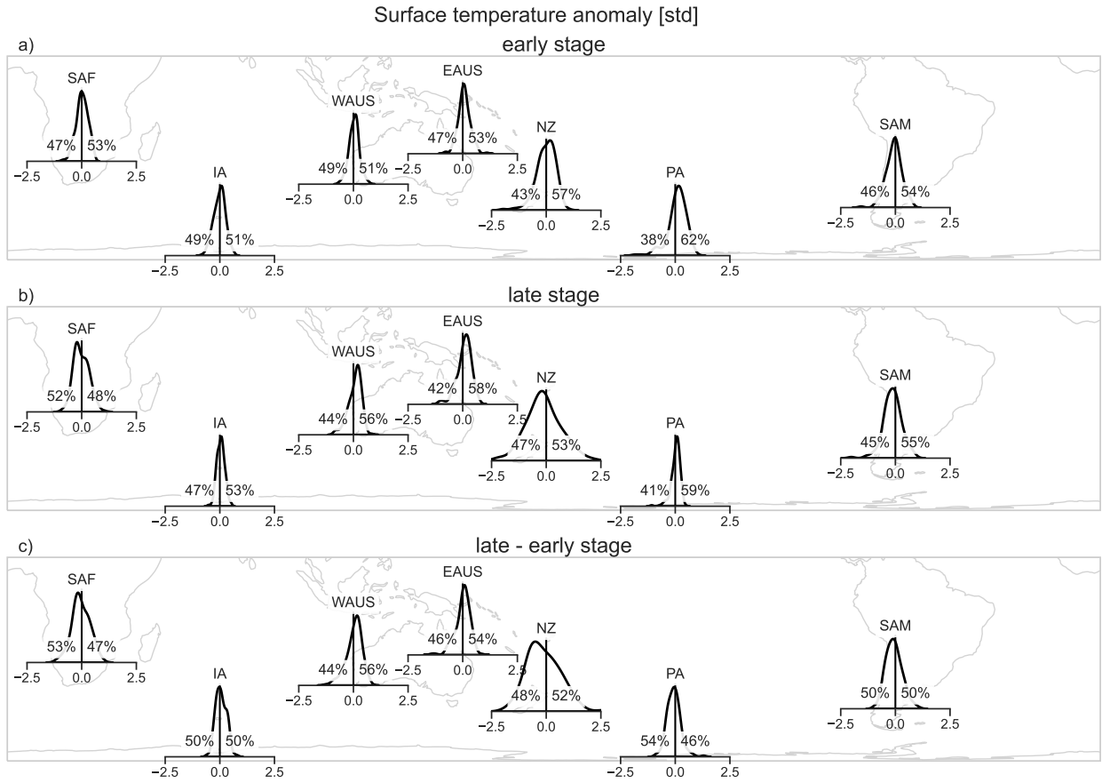
FIG. A3. Same as Fig. A3 but for years without SSWs. Given the PDFs show anomalies, their mean values are all zero and are therefore removed from the inset titles.
