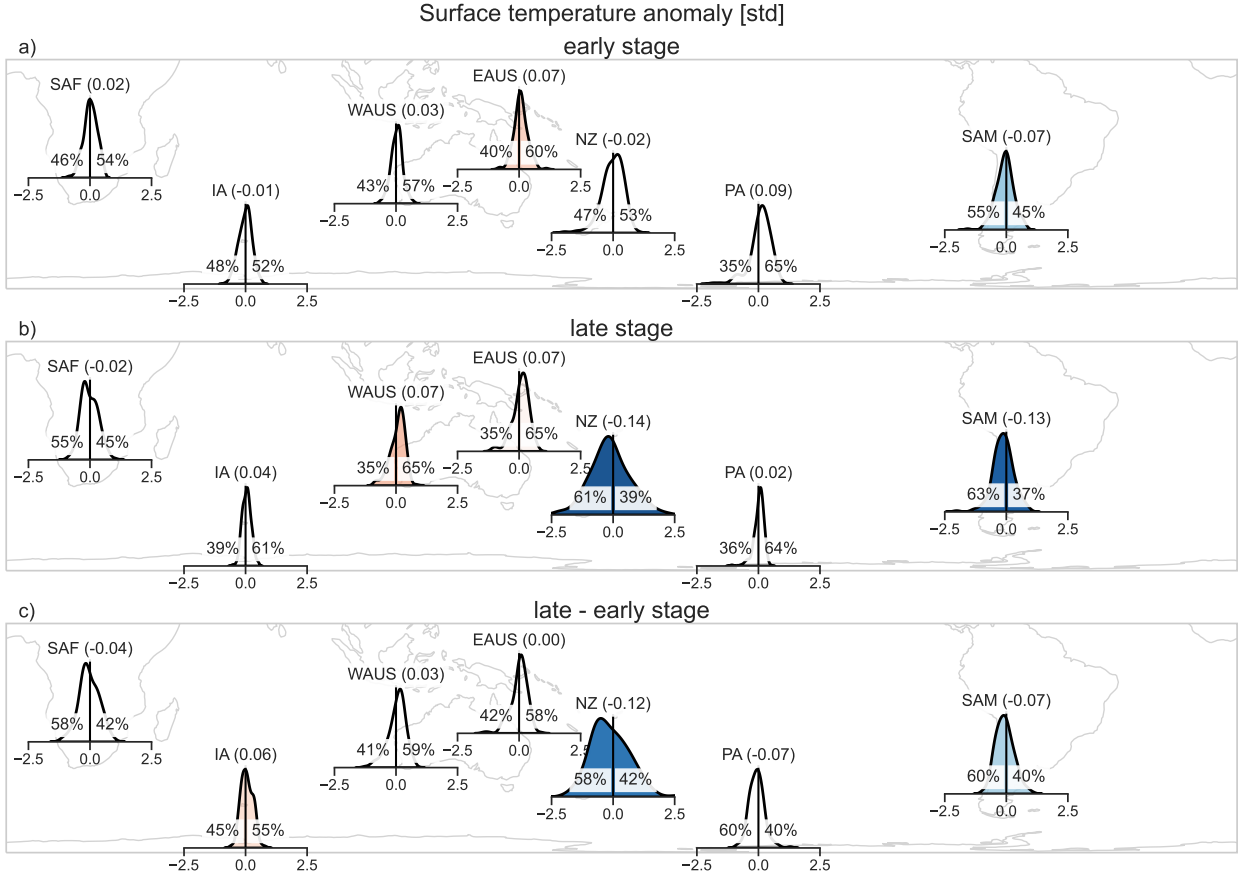
FIG. 4. Same as Fig. 3 but for standardized surface temperature anomalies. Red means warmer and blue cooler than usual on average.
