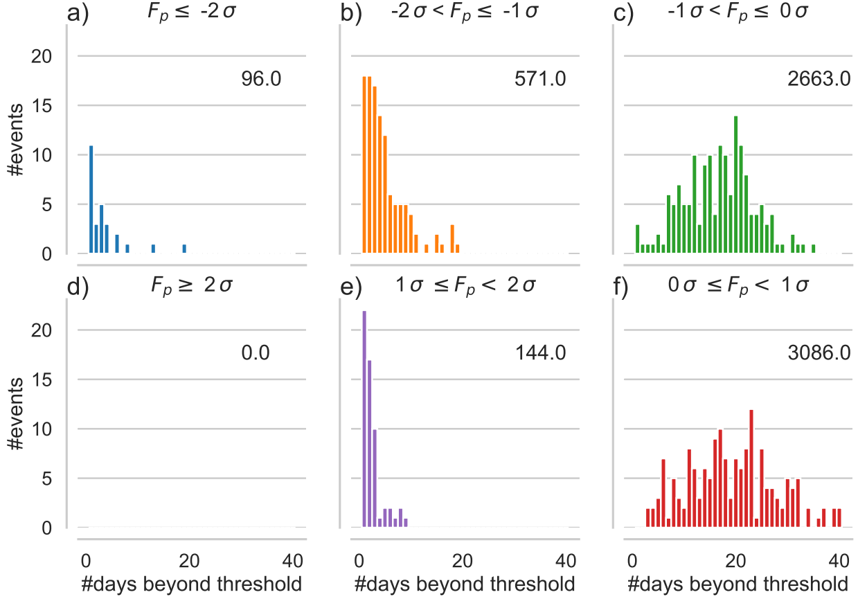
FIG. 7. Histograms of number of days spent within given threshold ranges (titles) of hemispheric-mean upward EP flux F_p during the early SSW stage (lags -60 to -20, i.e. 40 days) at 700 hPa. Top row shows upward anomalies, bottom row downward anomalies. The numbers in each panel give the total event days, i.e. the integral below each histogram. The total number of events is 161. The histograms suggest that the significant upward mean near the surface in Fig. 6b is due to individual periods of strong upward F_p (beyond 1\sigma ), which typically last for 1-2 weeks (panels a,b). In contrast, moderate to weak events (below 1\sigma ) are more evenly distributed between either sign (panels f,c).
