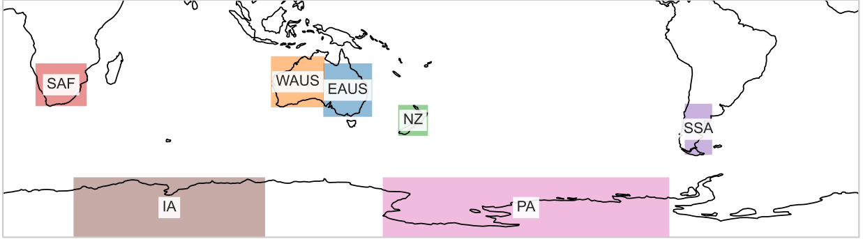
FIG. A1. Rectangular regions used for producing the PDFs of Figs. 3 and 4.
