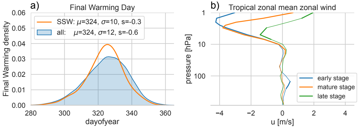
FIG. 13. (a) PDF of final warming date for (blue) all years and (orange) years with SSWs only. The legend includes information on mean day of year ( \mu ), standard deviation ( \sigma ) and skewness ( s ). (b) Composites of tropical mean ( 5^{\circ}\text{S} to 5^{\circ}\text{N} ) zonal mean zonal wind for the (blue) early, (orange) mature and (green) late stages. Thick lines mean anomalies are statistically significant at the 95% level.
