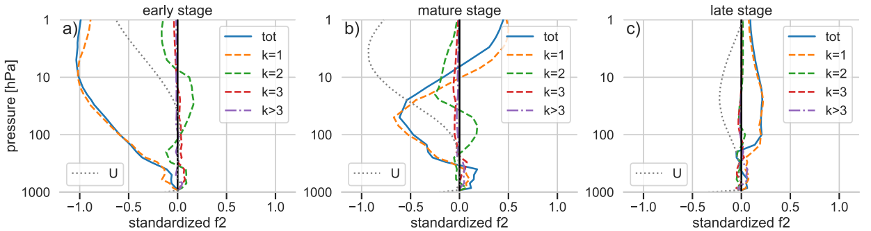
FIG. 8. Zonal mean zonal wind anomalies (gray dotted) and EP flux anomalies by wavenumber, divided into total EPz (blue, continuous), planetary wavenumbers 1-3 (colors, dashed), and synoptic scale waves (purple, dash-dotted). All quantities are area-weighted and averaged from 85-60S, and divided into the (a) early, (b) mature, and (c) late stages. Zonal mean zonal wind is plotted from -30 to +30 m/s (axis labels not shown), and the x-labels correspond to standardized EP fluxes.
