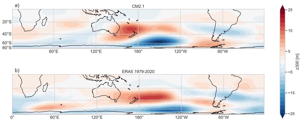
FIG. B2. Regression of TNI onto 300 hPa geopotential height in September-October-November for (a) CM2.1 and (b) ERA5 (1979-2020).
