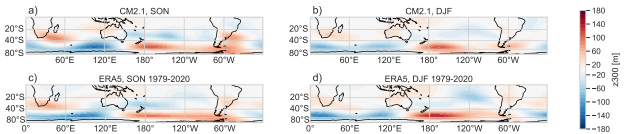
FIG. B4. 300 hPa stationary wave patterns for (top) CM2.1 and (bottom) ERA5 (1979-2020) during (left) September-October-November and (right) December-January-February. The model produces the stationary waves well, with similar amplitudes and only small biases in location of the lows and highs.
