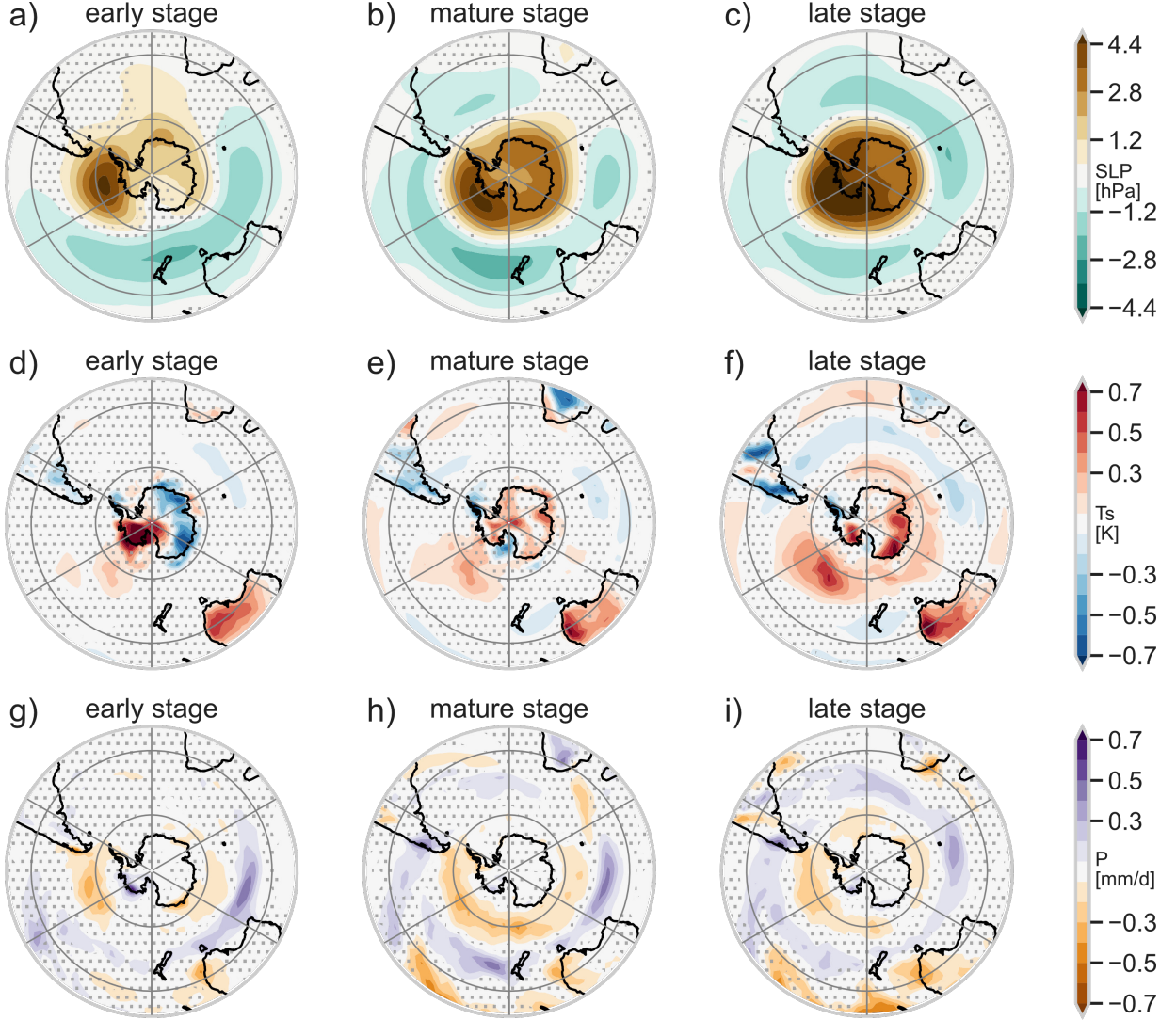
FIG. 1. Surface impact as measured by a)-c) sea level pressure, d)-f) surface temperature, and g)-i) precipitation, grouped into three 40-day lag periods (panel titles) corresponding to (left) early, (middle) mature and (right) late stages. For all variables, the hatches denote regions where the anomalies are not significantly different from zero based on a two-tailed t -test at the 95% level.
