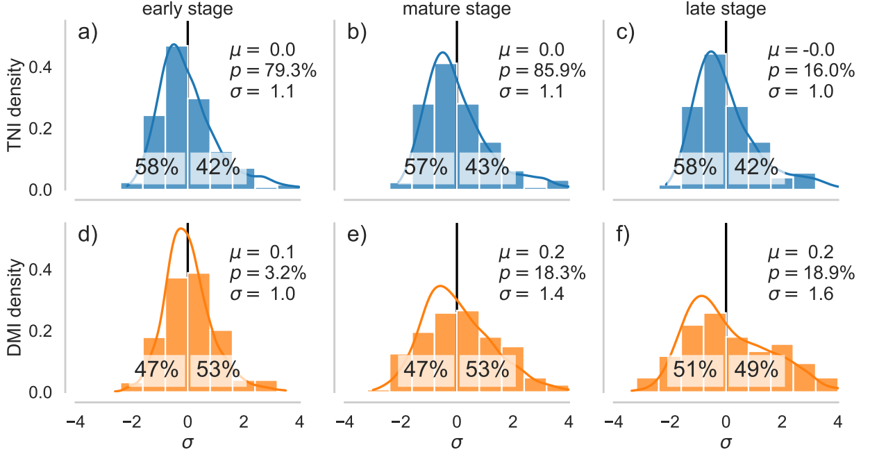
Fig. 5. PDFs of (a-c) ENSO via the Trans-Niño Index (TNI) and (d-f) the IOD via the Dipole Mode Index (DMI) for (left) early, (middle) mature, and (right) late stages. The bars represent histograms of all SSWs, while the continuous lines represent kernel density estimates (KDEs) from 1610 randomly chosen non-SSW years with the same seasonal distribution as the SSWs. As in Figs. 3 and 4, the percentages show the fraction of SSWs with negative or positive sign. The mean value of each PDF is denoted \mu and the p -value corresponds to a two-sided Kolmogorov-Smirnov test comparing the SSW (bars) to the climatological distributions (lines).
