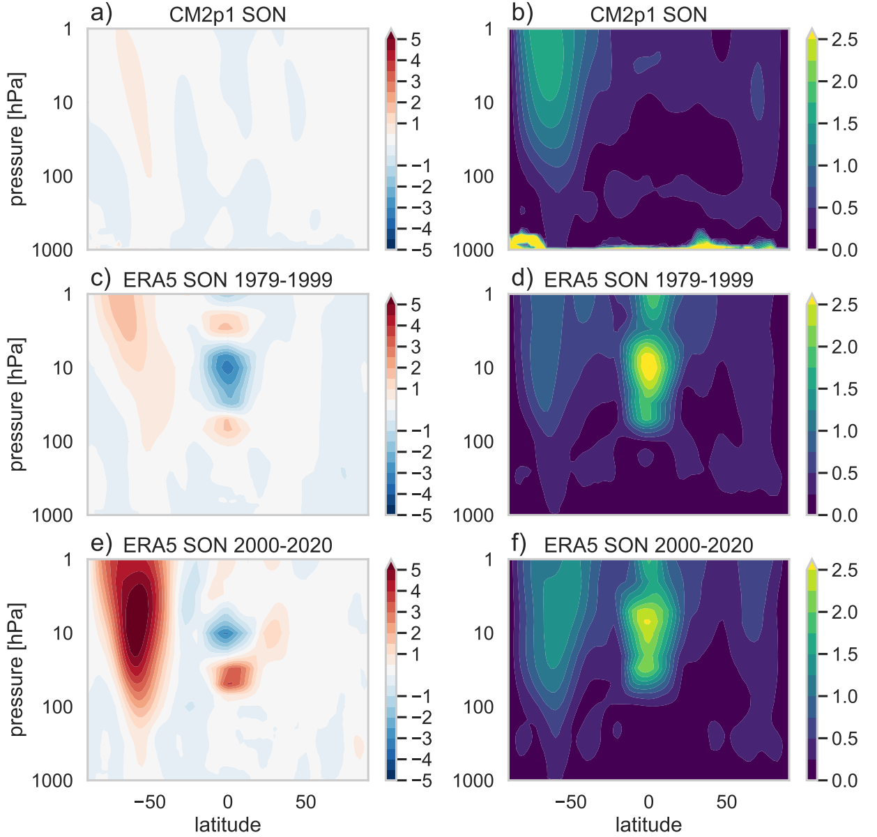
FIG. B3. (left) Regressions of monthly TNI on monthly zonal mean zonal wind anomalies during September-October-November in (a) CM2.1 and (c,e) ERA5. We have split the satellite reanalysis period into two equally long sub-periods (of 21 years) to illustrate the strong variability in the signal. Model regressions are similar to the earlier period in ERA5, but weaker than the later ERA5 period. In the tropics, ERA5 shows a QBO-like structure which is missing in the model. (right) Standard deviation of the same regressions using bootstrap re-sampling for (b) CM2.1 and (d,f) ERA5 (see text for details).
