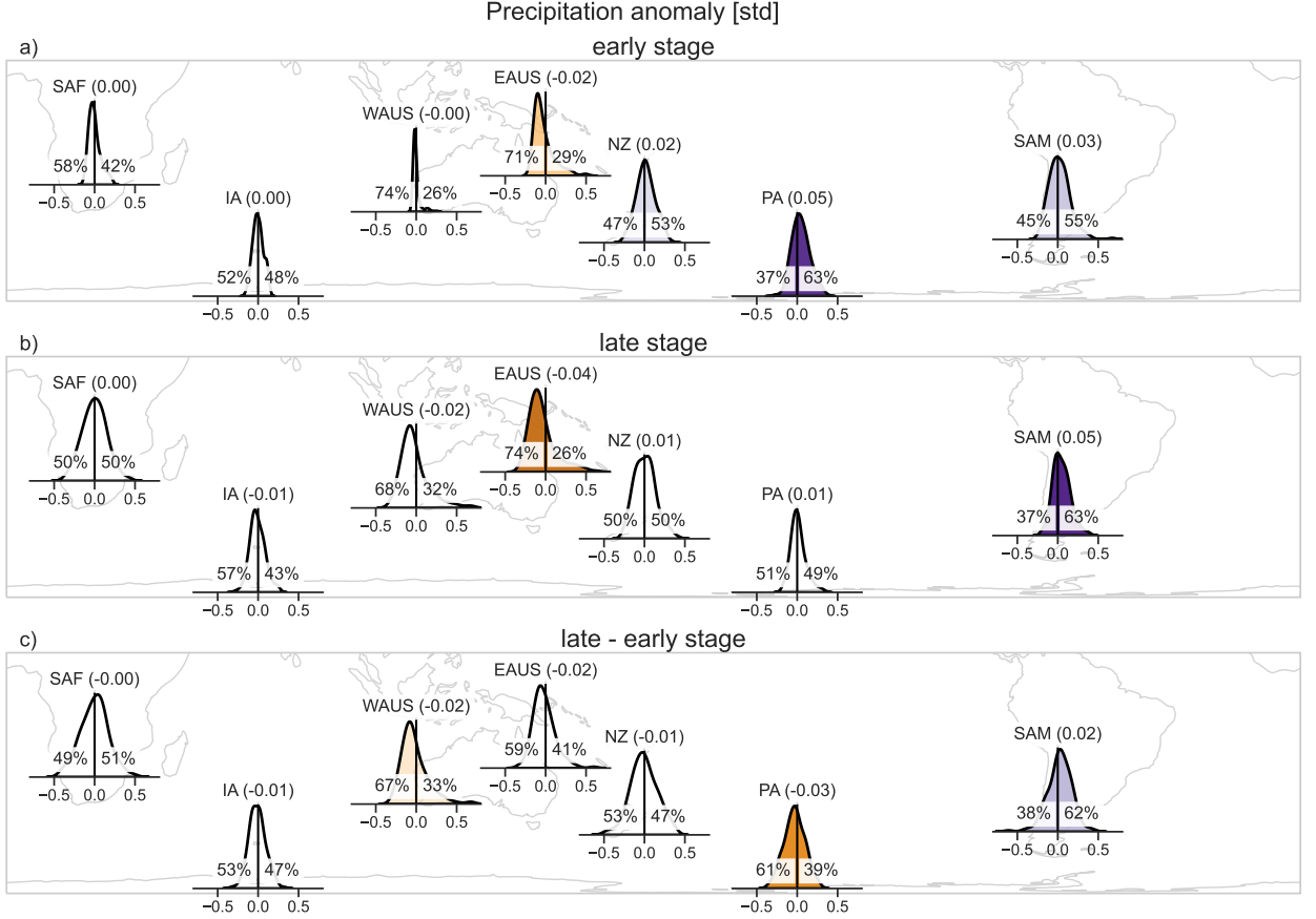
FIG. 3. PDFs for (a) early stage and (b) late stage standardized precipitation anomalies for different regions in the Southern Hemisphere. (c) shows the PDFs of precipitation change between the late and early stages. x -axis is labeled in units of standard deviation (by day of year), and the percentages show the fraction of events with positive or negative values. Numbers in the title show the means. Color according to mean value, with brown/orange drier and blue wetter than usual. Color is made transparent linearly with p -value from a Kolmogorov-Smirnov test if the actual distribution is distinct from a distribution sampled from 1610 non-SSW years (i.e. PDFs with associated p -values of more than 10% are not filled). The distributions were estimated using a Kernel Density Estimate (KDE). See Appendix A for the definitions of each region and significance testing.
