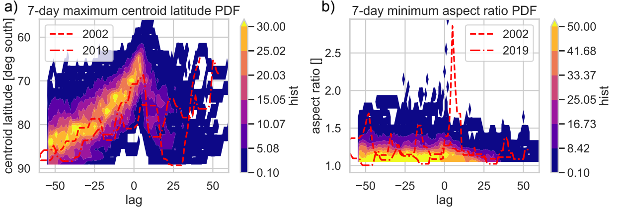
FIG. 12. Evolution of the PDF of (a) centroid latitude and (b) aspect ratio as a function of lag. As in Fig. 11 the 2019 event follows the model distribution very closely.
