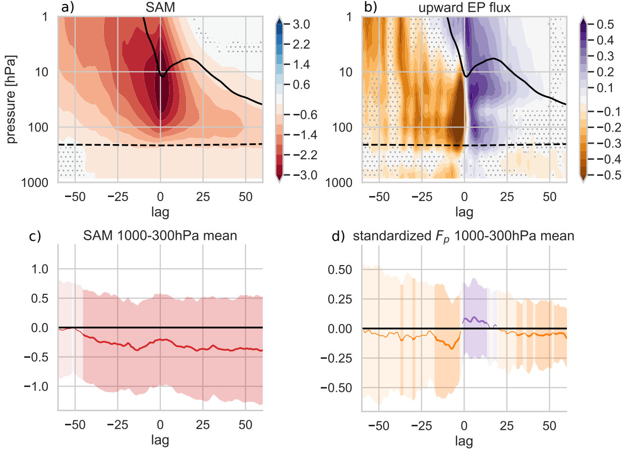
FIG. 6. Lag-pressure composites of (left) Southern Annular Mode index and (right) standardized vertical wave-one EP flux (negative means upward). The solid black line in (a) and (b) shows the zero contour of zonal mean zonal wind averaged between 70 and 50°S, and the dashed line shows the tropopause averaged between 90 and 20°S. EP flux is computed following Jucker (2021b) and standardized at each pressure level following Jucker (2016), cosine-latitude weighted and averaged from 20-90 S. Statistically insignificant regions (95% level) are hatched. The bottom panels show vertically averaged values between 1000-300hPa for the mean (bold) and cross-event standard deviation (shading). Not significant anomalies are drawn with lighter shading and a thin line.
