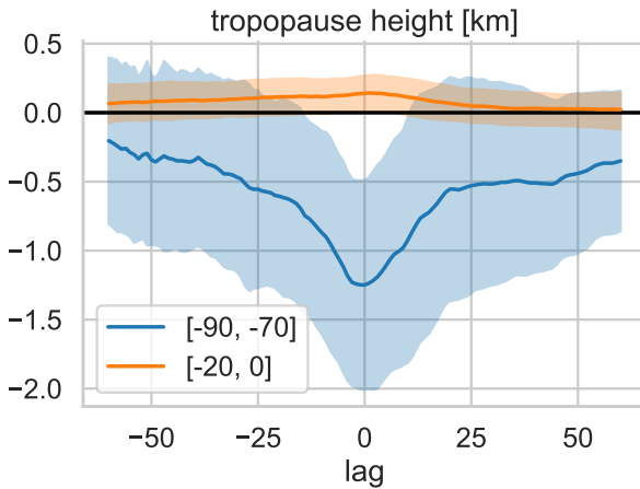
FIG. 10. Tropopause height anomalies as a function of lag for low latitudes ( 20^\circ\text{S} to the equator, orange) and high latitudes ( 90\text{--}70^\circ\text{S} , blue). Solid lines show the mean and shading the standard deviation across events. Tropopause calculated following Reichler et al. (2003).
