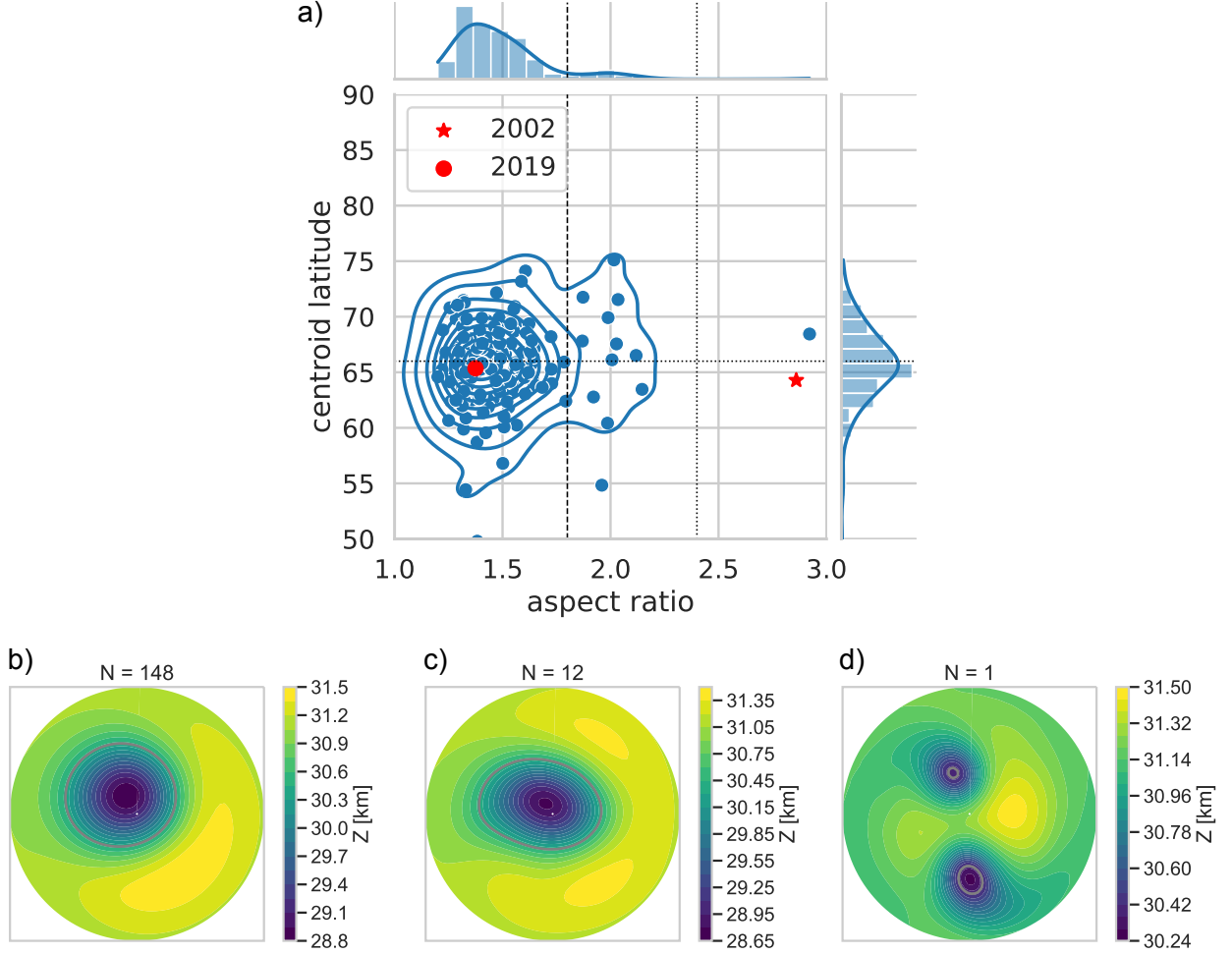
FIG. 11. 2D vortex moment analysis for all SSWs. (a) Distribution in aspect ratio - centroid latitude space, showing an almost Gaussian distribution around an aspect ratio of about 1.4 and a centroid latitude of 66^{\circ} S, which is similar to the observed 2019 minor SSW (red circle). Blue dots show a scatter plot of individual events and lags, while the blue contours define a Kernel Density Estimate of the same data. Thin gray dotted lines show the thresholds of 2.4 and 66^{\circ} S from Seviour et al. (2013) for the definition of split and displacement events in the Northern Hemisphere. In our analysis of the SH, there seems to be a secondary population of aspect ratios between 1.8 (black dashed line) and 2.4 (gray dotted vertical line). The composite of the population with aspect ratios below 1.8 is shown in (a) and corresponds to displacement events. Events with aspect ratios between 1.8 and 2.4 is shown in (b), which does not correspond to a split vortex per se, but includes two distinct geopotential height maxima around 30^{\circ} E and 150^{\circ} E (panel c). There is only one single event in the simulation similar to the vortex split of 2002 (aspect ratio above 2.4, panel d). The composites in panels b-d are created by averaging over all events and lags where the respective conditions on aspect ratio are satisfied. The solid gray lines show the 30.4 km lines used to detect the vortex edge in the momentum calculations, and the title shows the number of events in the composite.
