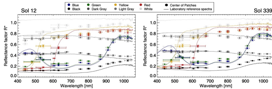
Figure 6. Calibration Target spectra from sol 12 and 339. The circles are the observed calibrated R^* reflectances of the clean spots, while the solid lines represent the corresponding laboratory spectra.
