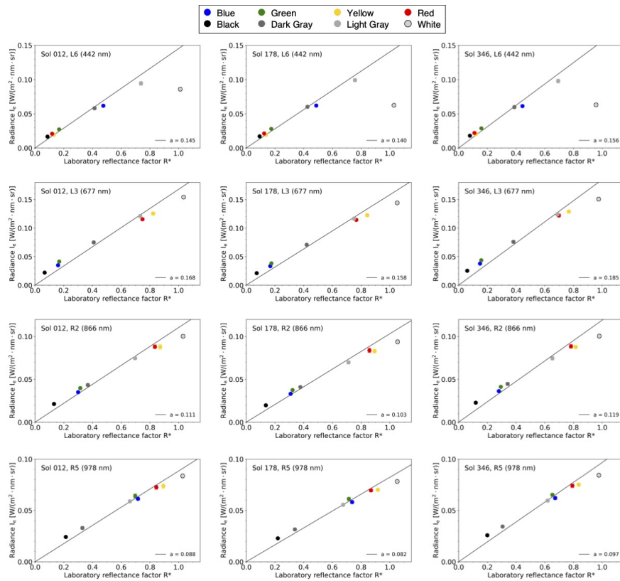
Figure 5. Examples of one-term linear fits (in the form y = a \bullet x ) over the data points of measured radiance and model reflectance factor for three sols (sol 12, 178, 346, along the columns) in four filters (L6, L3, R2, R5, along the rows). The straight black lines are the fits. All the eight clean spots are plotted, but the white was not used to compute the fits.
