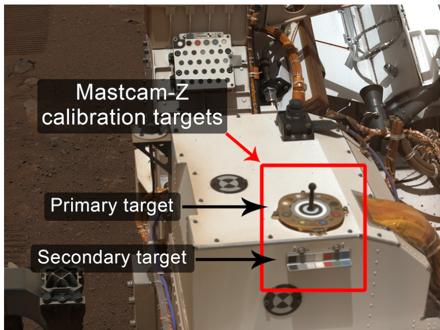
Figure 1. Context image of the Mastcam-Z primary and secondary calibration targets, taken by the left eye of Mastcam-Z (L0) on sol 23 at 26 mm focal length (Image-ID: ZL0_0023_0668982043_910IOF_-N0030770ZCAM03003_0260LMA01, sequence ZCAM03003). In the upper center, the SuperCam calibration target is also visible.
