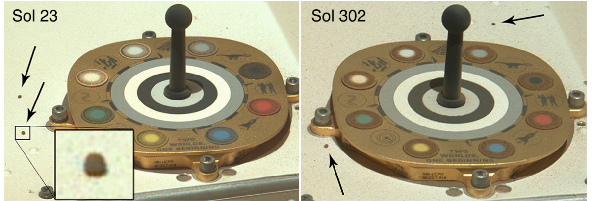
Figure 14. Primary target imaged by the left eye of Mastcam-Z (a) on sol 23 at 100 mm focal length (seq. ZCAM03014) and (b) on sol 302 at 48 mm focal length (seq. ZCAM03014) with the presence of large sand grains indicated by arrows. (c) One of the grains in the sol 23 image is magnified for better display. Image-IDs: (a) ZLF_0023_0668983099_596FDR_N0030770ZCAM03003_1000LMJ, (b) ZL0_0302_0693748246_223ECM_N0090000ZCAM03014_048085J.
