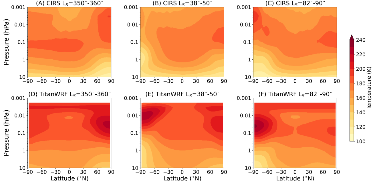
Figure 1: Zonally averaged temperature from CIRS (A-C) and TitanWRF (D-F) at southern autumn equinox (left), southern mid-autumn (middle), and southern winter solstice (right). Values are only shown here and in the following figures for the 10 hPa - 0.001 hPa range to focus on behavior in the stratosphere and mesosphere.
