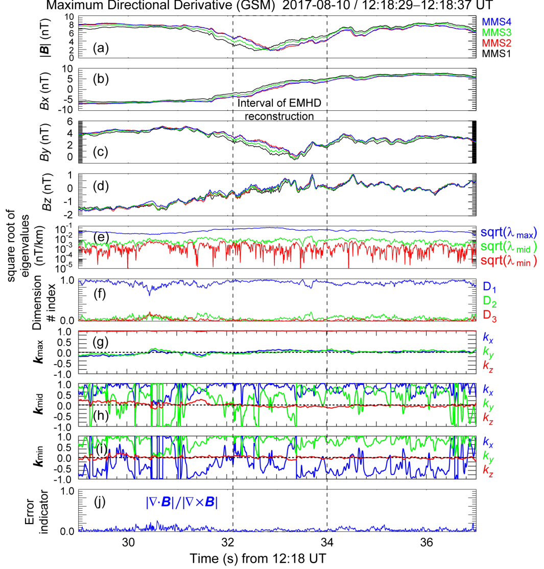
Figure 3. Results from the MDD method (Shi et al., 2019) applied to an interval 12:18:29–12:18:37 UT. (a-d) GSM components of the magnetic field measured by the four MMS spacecraft (a; |\mathbf{B}| , b; B_x , c; B_y , d; B_z ). (e) Square roots of the maximum, intermediate, and minimum eigenvalues ( \lambda_{\max} , \lambda_{\text{mid}} , \lambda_{\min} ) of the 3 \times 3 MDD matrix (Shi et al., 2019). (f) Dimension number indices (Rezeau et al., 2018), defined as D_1 = \frac{(\lambda_{\max} - \lambda_{\text{mid}})}{\lambda_{\max}} , D_2 = \frac{(\lambda_{\text{mid}} - \lambda_{\min})}{\lambda_{\max}} , and D_3 = \frac{\lambda_{\min}}{\lambda_{\max}} , that can be used as measures of the dimensionality of the structure encountered by the spacecraft. (g-i) Eigenvectors corresponding to the three eigenvalues (g: k_{\max} ; h: k_{\text{mid}} ; i: k_{\min} ). (j) \frac{|\nabla \cdot \mathbf{B}|}{|\nabla \times \mathbf{B}|} as an error proxy.
