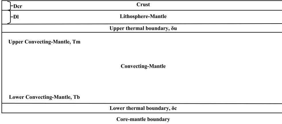
Figure A1. The disproportionate schematic diagram of the 1-D global parametric model of Mercury. This model radially divides the planet into several layers: the crust, lithosphere-mantle, upper/lower thermal boundary, convecting mantle and the outer/inner core (not displayed).
