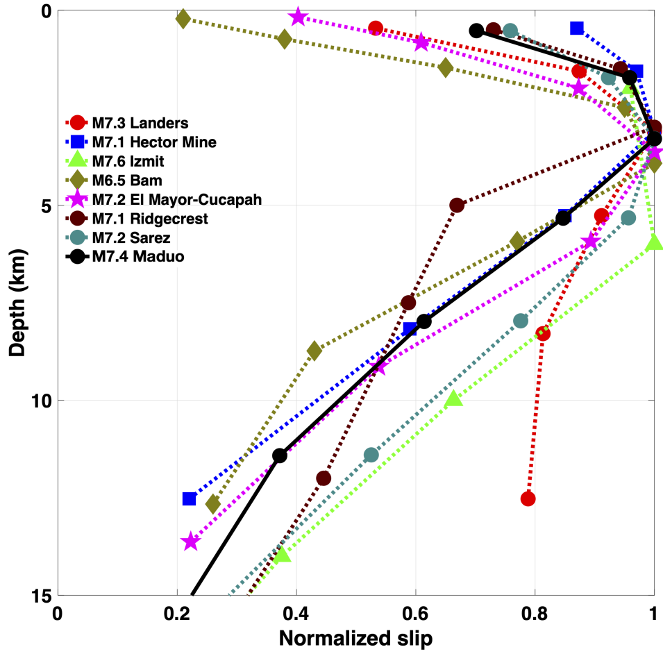
Figure 4. Along-strike averaged normalized coseismic slip as a function of depth for the 2021 M7.4 Maduo earthquake (black solid line), as well as for several other M~7 strike-slip earthquakes (color dashed lines, data from Fialko et al. (2005); Jin and Fialko (2020)).
