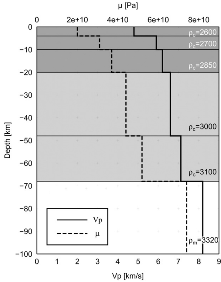
Figure S4: One-dimensional rigidity structure of the north-eastern Tibet used in our layered elastic half-space models. Top horizontal axis: shear modulus \mu , bottom horizontal axis: P-wave velocity V_p . \rho_c and \rho_m are the densities of the Earth's crust and mantle, respectively, in kg/m 3 . From Xiong, Shan, Zheng, and Wang (2010).
