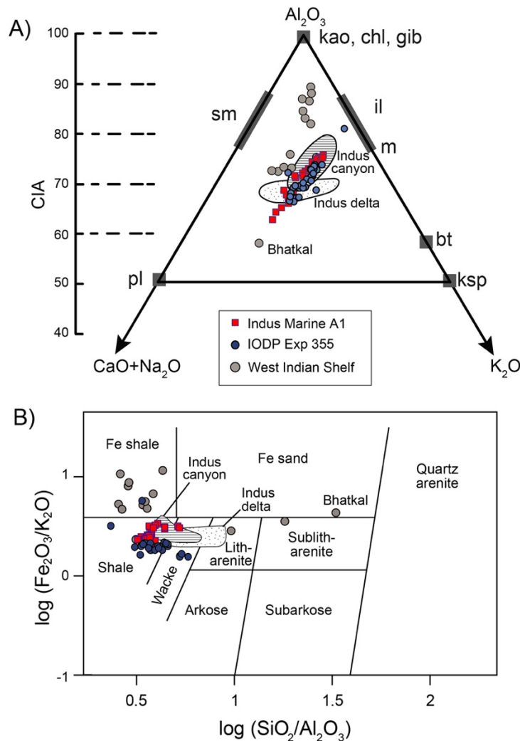
381 Figure 5. (A) Geochemical signature of the analyzed samples illustrated by a CN-A-K ternary 382 diagram [Fedo et al. , 1995]. CN denotes the mole weight of Na_2O and CaO^* ( CaO^* represent the 383 CaO associated with silicate, excluding all the carbonate). A and K indicate the content of Al_2O_3 384 and K_2O respectively. Samples closer to A are rich in kaolinite, chlorite and/or gibbsite 385 (representing by kao, chl and gib ). CIA values are also calculated and shown on the left side,
