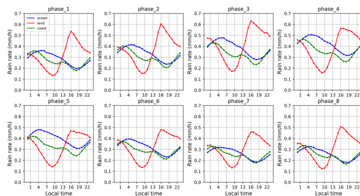
Figure S6. The diurnal cycle of rain rate over the Maritime Continent during MJO phases 1-8.
