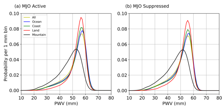
Figure S7. The probability density function (PDF) of PWV over the Maritime Continent during (a) active MJO phases and (b) suppressed MJO phases.
