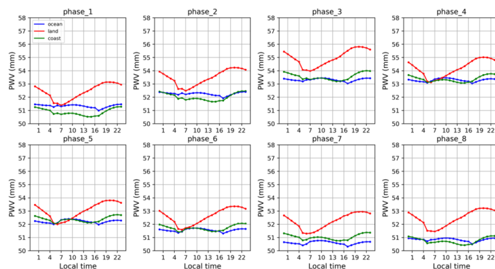
Figure S5. The diurnal cycle of precipitable water vapor over the Maritime Continent during MJO phases 1-8.
