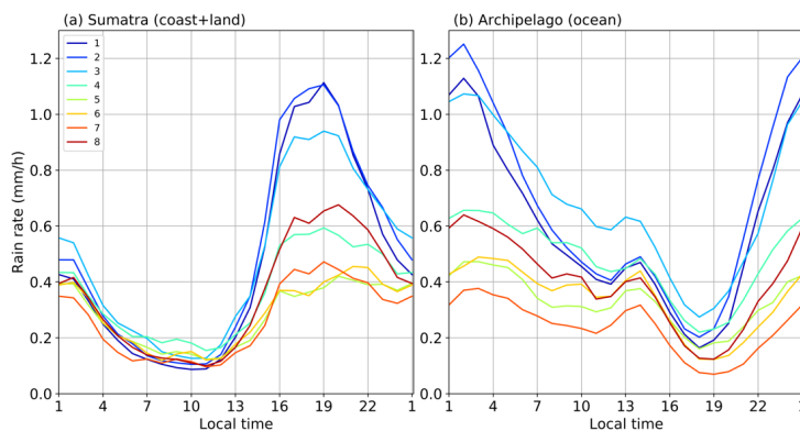
Figure S4. The diurnal cycle of precipitation rate over SuGAR stations (2008-2013) during MJO phases 1-8 (color), for (a) coast and land stations, and (b) ocean stations.
