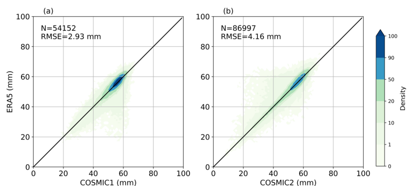
Figure S1. 2D histograms of ERA5 reanalysis PWV data with (a) COSMIC1 and (b) COSMIC2.
