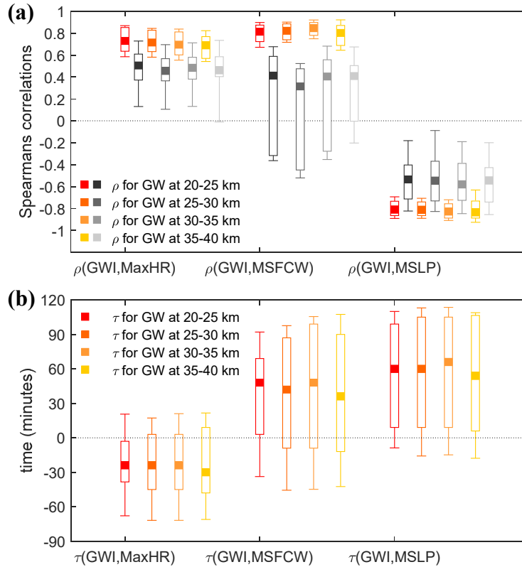
Figure 4. Spearman correlation coefficients and time lag between variable series. (a) Spearman correlation coefficients \rho between the GWI and MaxHR, MSFCW, and MSLP, respectively. The original \rho is marked in black and grey, and the time-lagged \rho is marked in orange. (b) The “best” time lag \tau between GWI and MaxHR, MSFCW, and MSLP, respectively. The box plot displays the minimum, first quartile (25%), median, third quartile (75%), and maximum values.
