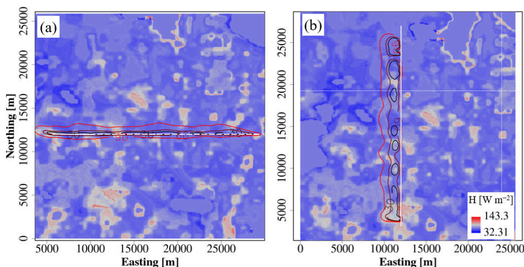
485 Figure 12. Example virtual flight tracks and their 30%, 60% and 90% source area contours superimposed over the LES sensible heat flux surface forcing ( \text{W m}^{-2} ). (a) Wind-parallel flights sample source areas that are elongated along the flight track leading to considerable overlap. (b) Wind-perpendicular flights sample less overlapping source areas along the flight track, and thus capture more independent samples and spatial variability.
