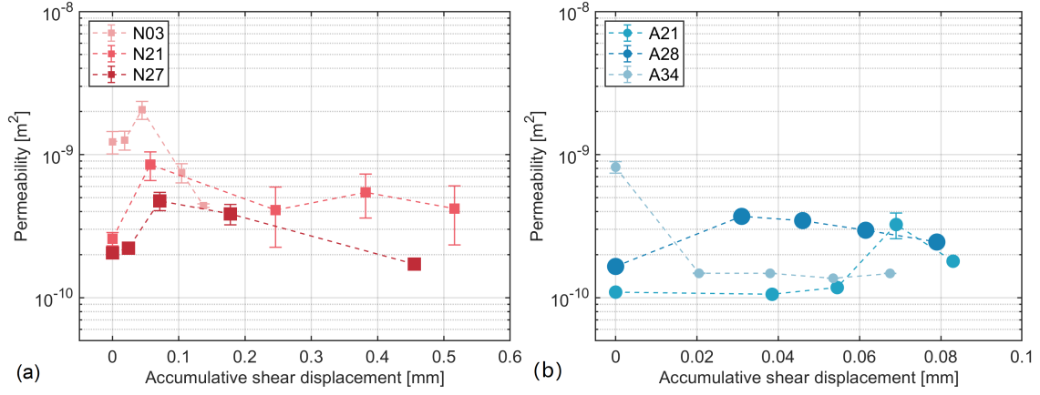
Figure 7: Relationship between calculated permeability, k , and accumulated shear displacement, \sum d_i for (a) natural and (b) saw-cut fractures. The fluctuations in measured permeabilities, indicated by the vertical error bar, given as standard deviation. Note the different scale of the accumulative shear displacements for natural and saw-cut fractures. Specimens with larger roughness values are marked by bigger markers.
