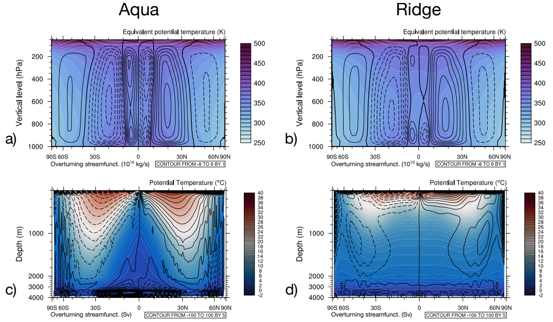
Figure 8. Zonally averaged vertical sections, 100-yr climatology: (a–b) Atmosphere: Eulerian meridional overturning streamfunction ( 10^{10} \text{kg s}^{-1} , contour lines; solid is positive/clockwise, dashed is negative/counterclockwise), overlaid on equivalent potential temperature (K, colored shading); (c–d) Ocean: residual overturning streamfunction (Sv, contour lines; solid is positive/clockwise, dashed is negative/counterclockwise), overlaid on potential temperature ( ^{\circ} C, colored shading). The overturning cells in the ocean are closed to within the magnitude of atmospheric moisture transport in the surface mixed layer (see P-E in Fig. 4h).
