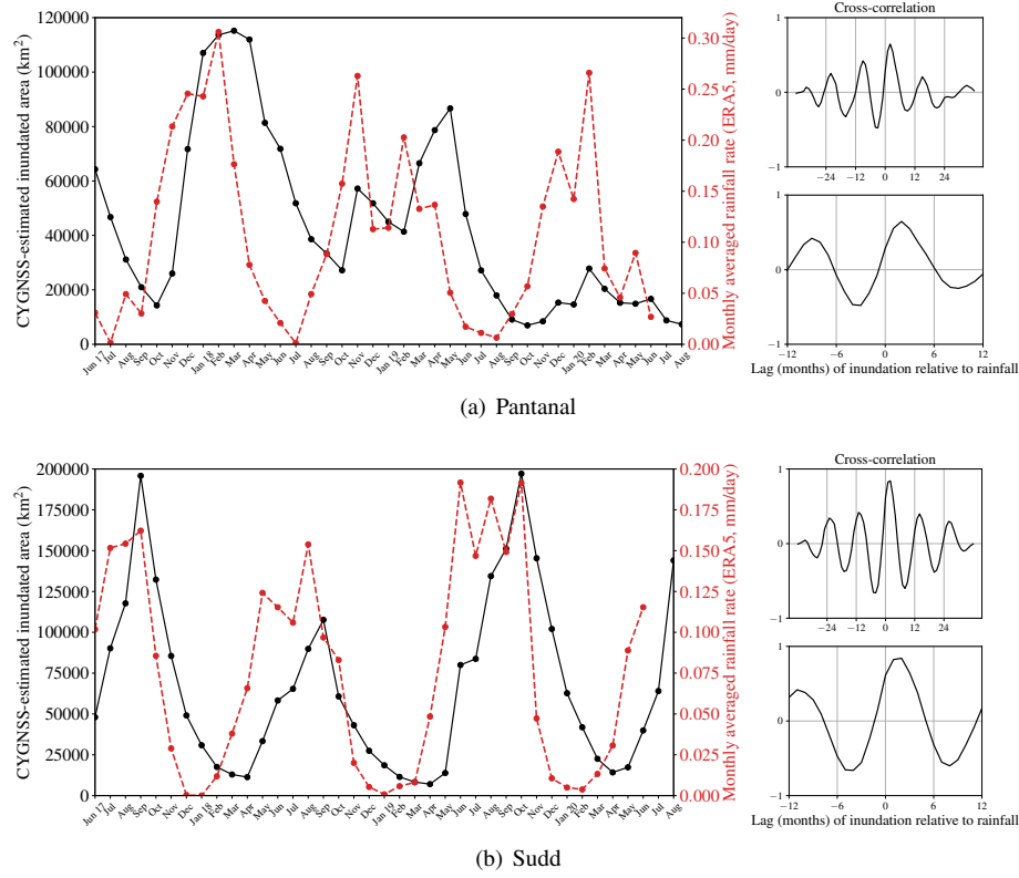
Figure 3: Monthly inundation extent (black solid lines) based on CYGNSS watermarks and monthly average rainfall rate from ERA-5 data (red dashed line) over (a) the Pantanal and (b) the Sudd. The figures on the right show the cross-correlations between rainfall and inundation extent, highlighting the one to two month lag between the two timeseries.
