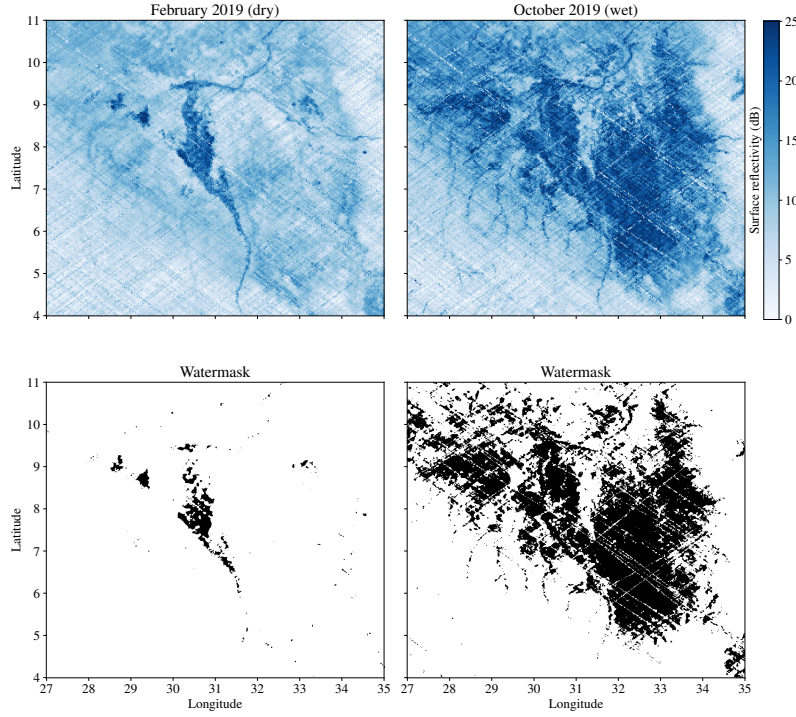
Figure 2: Inundation maps over the South Sudanese Sudd wetland for two different months of data ; left: February 2019 (dry season), and right: October 2019 (wet season). Top: surface reflectivity from CYGNSS. Bottom: final watermask obtained.
