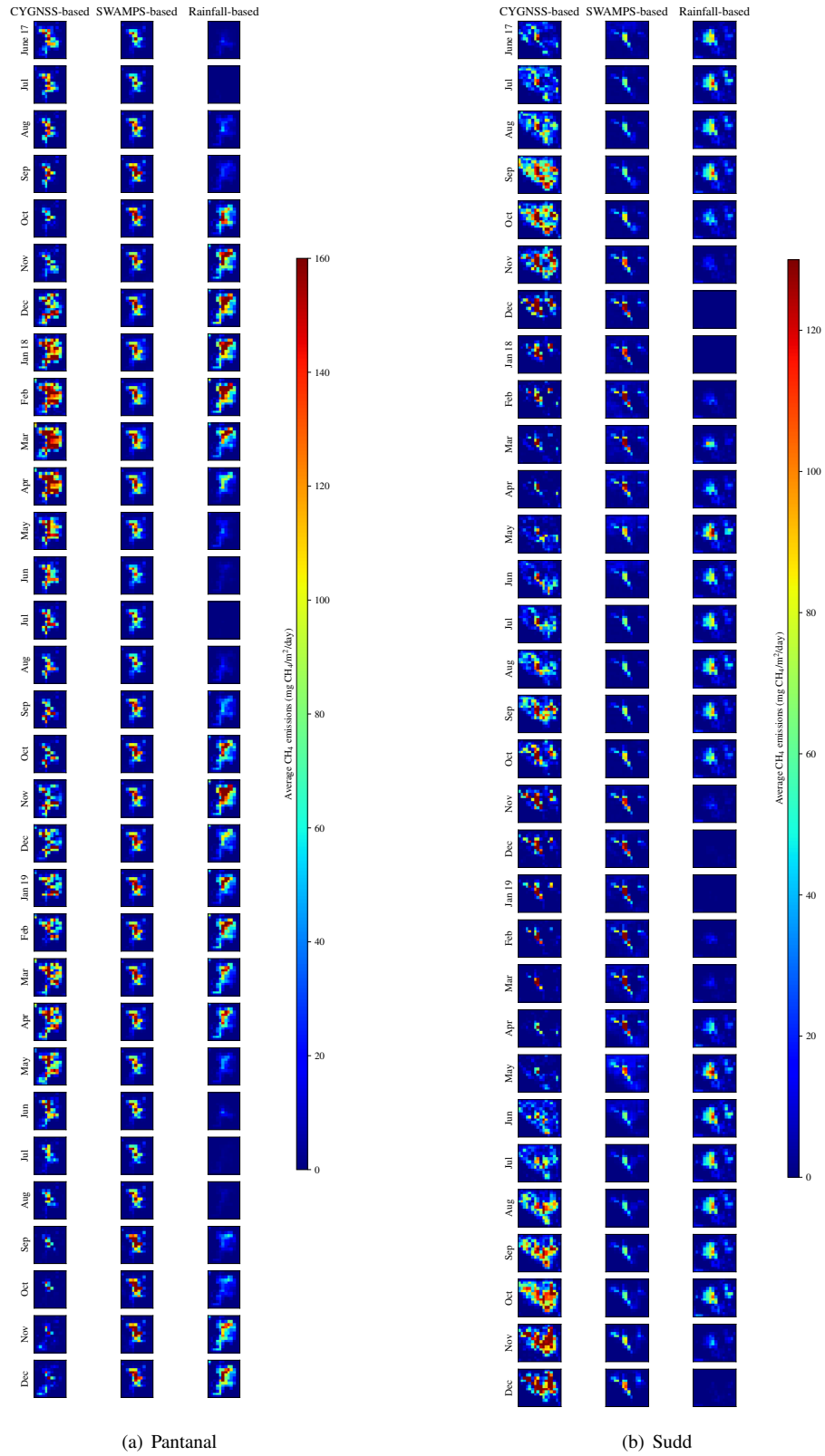
Figure S5: Average monthly emissions for (a) the Pantanal and (b) the Sudd wetlands based on CYGNSS inundation maps (left), SWAMPS inundation maps (center), and ERA5 rainfall (right).
