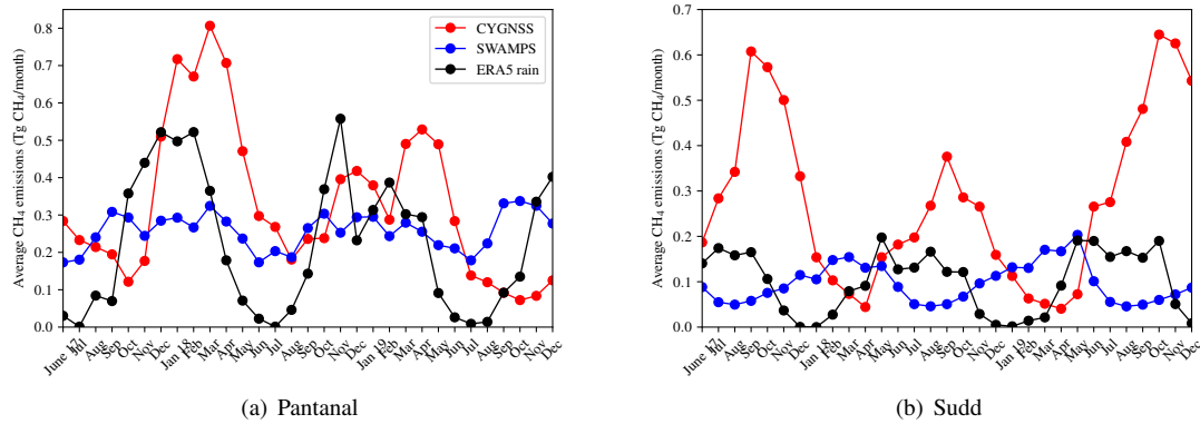
Figure S4: Average monthly emissions converted to Tg of \text{CH}_4 /months over the whole area for (a) the Pantanal and (b) the Sudd wetlands based on CYGNSS watermarks (red), SWAMPS maps (blue), and ERA5 rainfall (black). The lines show the average of all 18 models.
