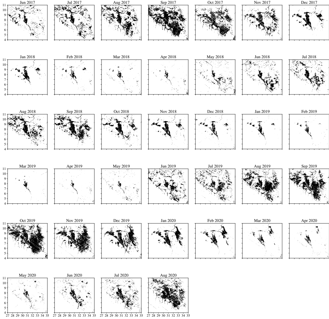
Figure S2: Monthly CYGNSS-based watermarks at 0.01^\circ \times 0.01^\circ resolution over the Sudd wetland in South Sudan.
