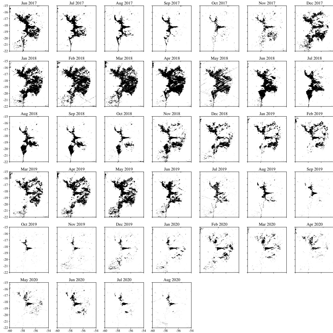
Figure S1: Monthly CYGNSS-based watermarks at 0.01^\circ \times 0.01^\circ resolution over the Pantanal wetland in Brazil.
