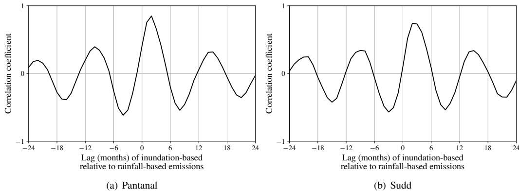
Figure 5: Cross-correlations between rainfall-based and inundation-based WetCHARTs \text{CH}_4 emissions, highlighting the two months lag between the two timeseries over (a) the Pantanal and (b) the Sudd wetlands.
