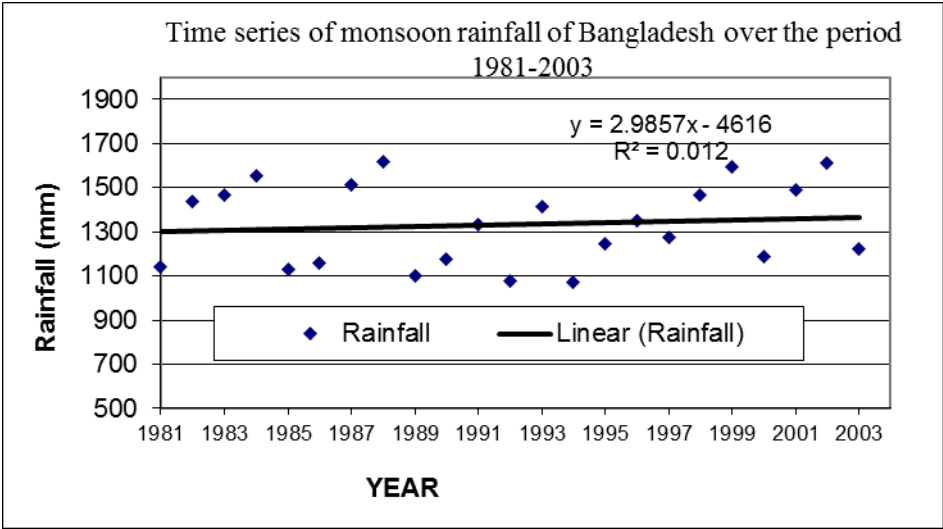
Fig. 10. Time series of monsoon rainfall of Bangladesh over the period 1981-2003
