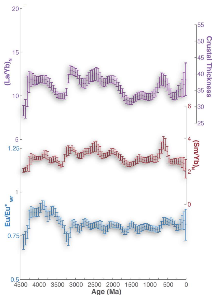
Figure 11. Global calculated whole rock \text{La/Yb}_n , \text{Sm/Yb}_n and \text{Eu/Eu}^* from zircon petrochronology (Balica et al., 2020). Crustal thickness over time is also shown on the right (as determined by Profeta et al., 2015 based on \text{La/Yb} ). 98% all analyzed zircons are from granitoid magmas (Balica et al., 2020). Diagram shows that to a first order, granitoids were fractionated out of magmatic systems at 35–45 km over time, similar to conditions required to make arclogitic roots. Mechanisms for fractionating or remelting basalts under lower crustal conditions may however have been different in the geologic past compared to modern arc settings (Balica et al., 2020).
