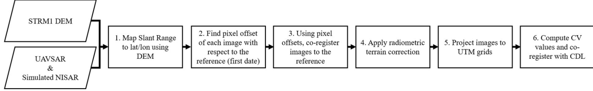
Figure 3. Flowchart showing the six data processing steps. Steps 1 through 5 were applied using the InSAR Scientific Computing Environment software via an automated workflow (ISCE Docker Tools).
