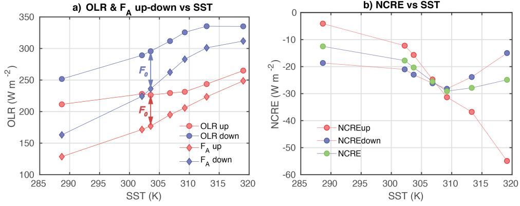
Figure 4. a) OLR and atmospheric cooling rate contribution to OLR from F_A and F_0 in the upward and downward regions as a function of global mean SST for the seven basic experiments. F_0 is the difference between OLR and F_A , as indicated by the arrows for case C303. b) Net Cloud Radiative Effect (NCRE) for upward, downward and global mean averages
