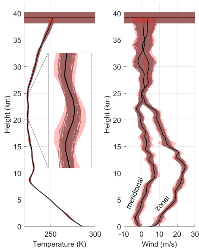
FIG. 2. Example of inversion initialization. The initial model consists of temperature and wind profiles, and reflection altitude (black lines). The solution space is bounded with a multiple of the standard deviations of the initial model parameters ( 5\sigma in this example) and a limit manually specified in the case of the reflection altitude (red shaded areas). The search is conducted with a swarm of 96 particles whose initial position is determined by solutions (smoothed profiles) selected at random within the limits of the solution space (grey lines).
