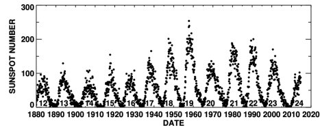
Figure 12: Number of Sunspots vs. time as an indicator of the Sun cycle (Hathaway, 2015).
