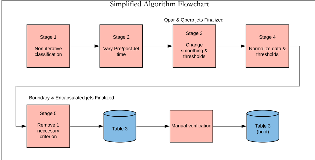
Figure A1. Simplified flowchart of the classification algorithm utilized to generate the dataset shown in Table 3.
